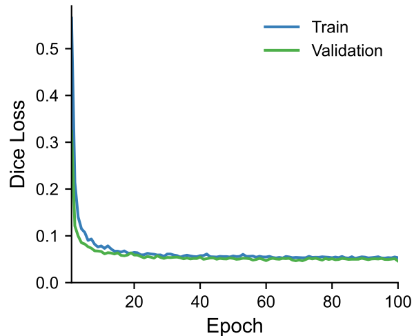
Training Loss
