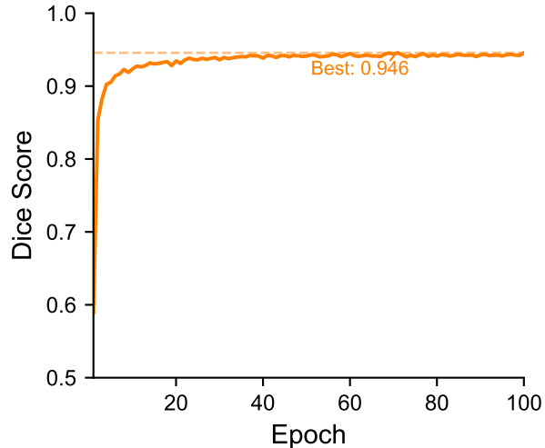
Validation Dice
