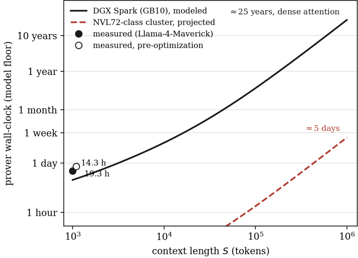
Figure 3: Figure 3: Prover wall-clock against context length: the modeled floor from the cost identity of Appendix A.5 on the demonstrated machine (solid), the measured runs of §9 (points), and the projection to an NVL72-class cluster (dashed), which divides the bandwidth-riding terms by the aggregate-bandwidth ratio while the column hashing rides hash throughput. Both curves assume dense attention in every layer.
