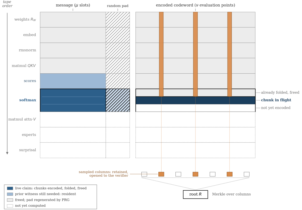
Figure 1: Figure 1: The streaming prover (§6.1, §6.3). Claims are committed in tape order: each row is encoded (left: message slots and zero-knowledge pad; right: codeword), folded into the column hashes and test-polynomial accumulators, then freed. Only the chunk in flight and prior witness still referenced stay resident. The Merkle tree is built over codeword columns; the audited columns are retained and opened to the verifier.
