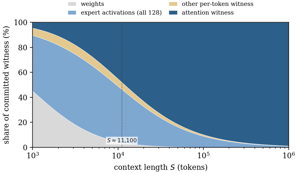
Figure 2: Figure 2: Composition of the committed witness for Llama-4-Maverick as context grows (Appendix A.4). Weights dominate below about 900 tokens, the committed experts from there to the second crossover at S \approx 11,100 , and attention above.
