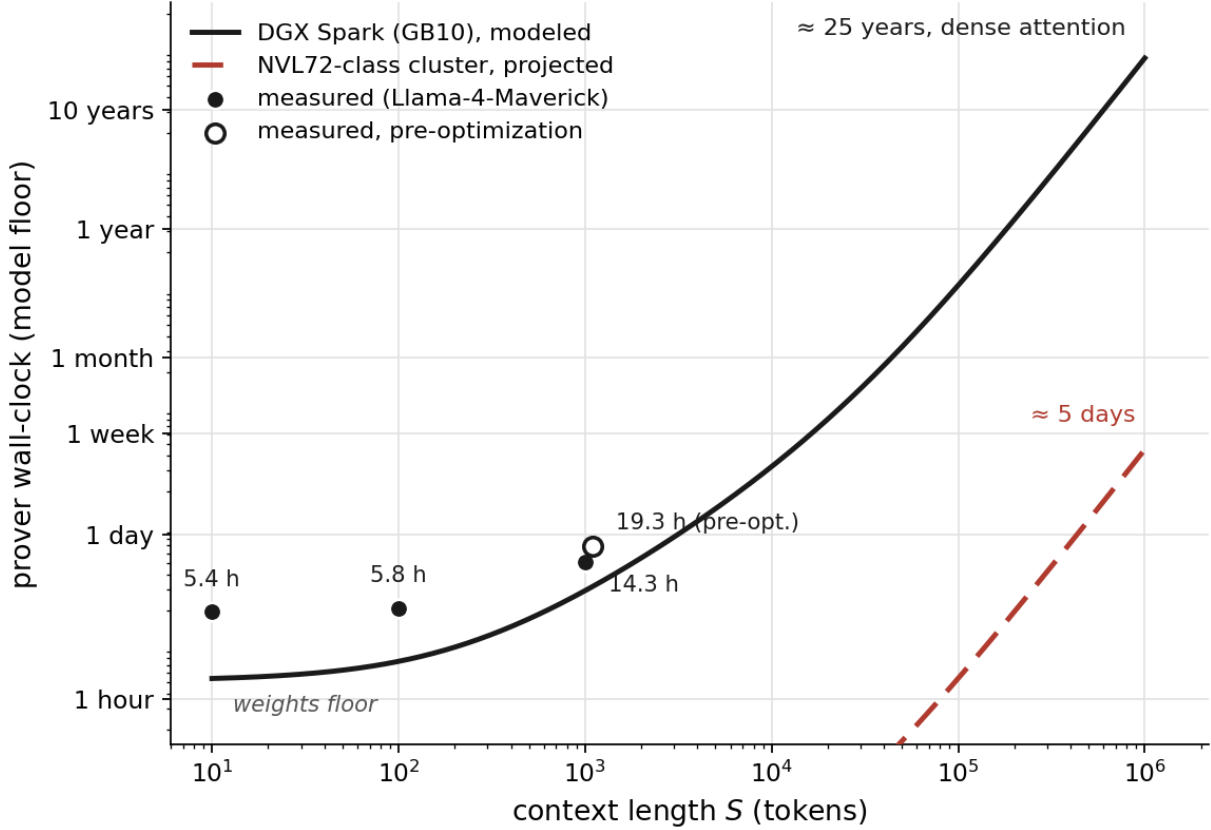
Figure 3: Prover wall-clock against context length: the modeled floor from the cost identity of Appendix A.5 on the demonstrated machine (solid), the measured runs of §9 (points), and the projection to an NVL72-class cluster (dashed), which divides the bandwidth-riding terms by the aggregate-bandwidth ratio while the column hashing rides hash throughput. Both curves assume dense attention in every layer; below the first crossover of §8 the curve is nearly flat on the weights floor.
