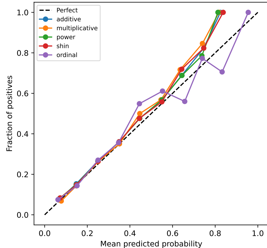
Away calibration
