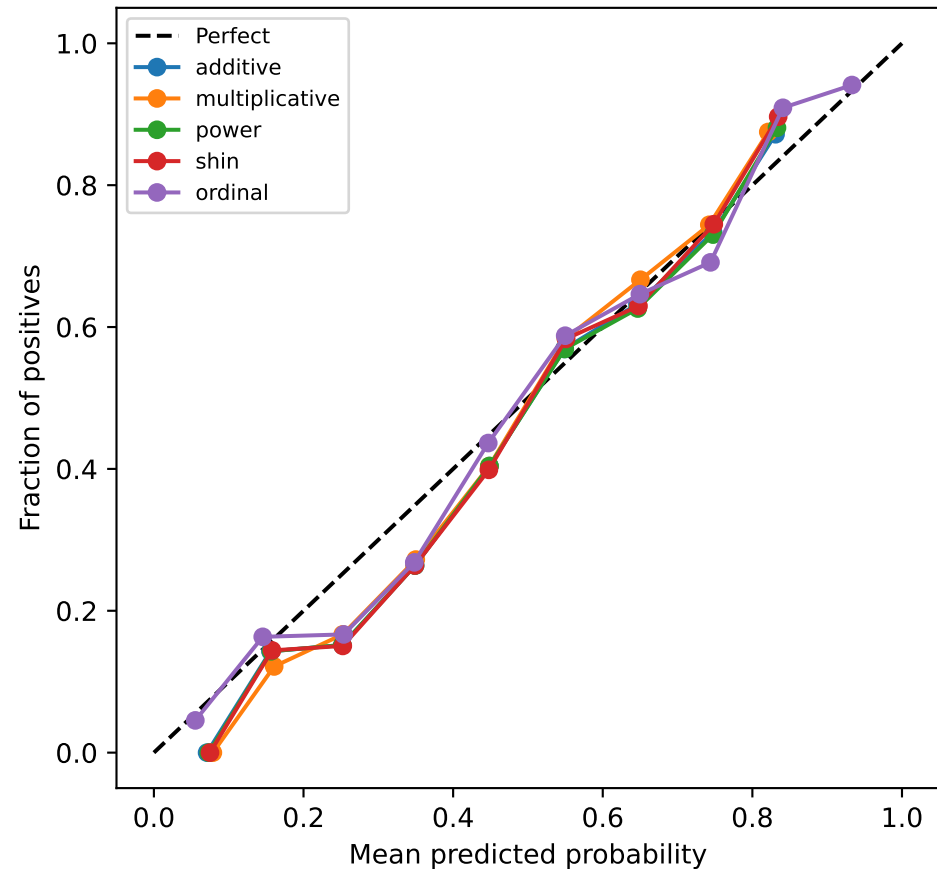
Home calibration
