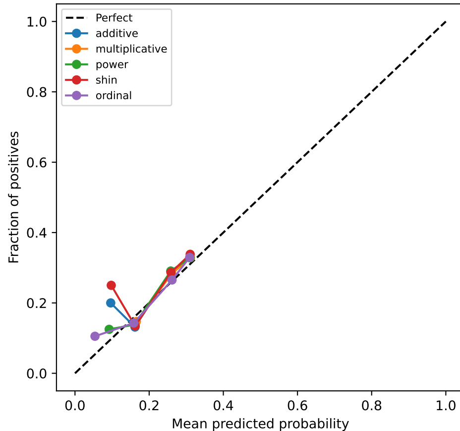
Draw calibration
