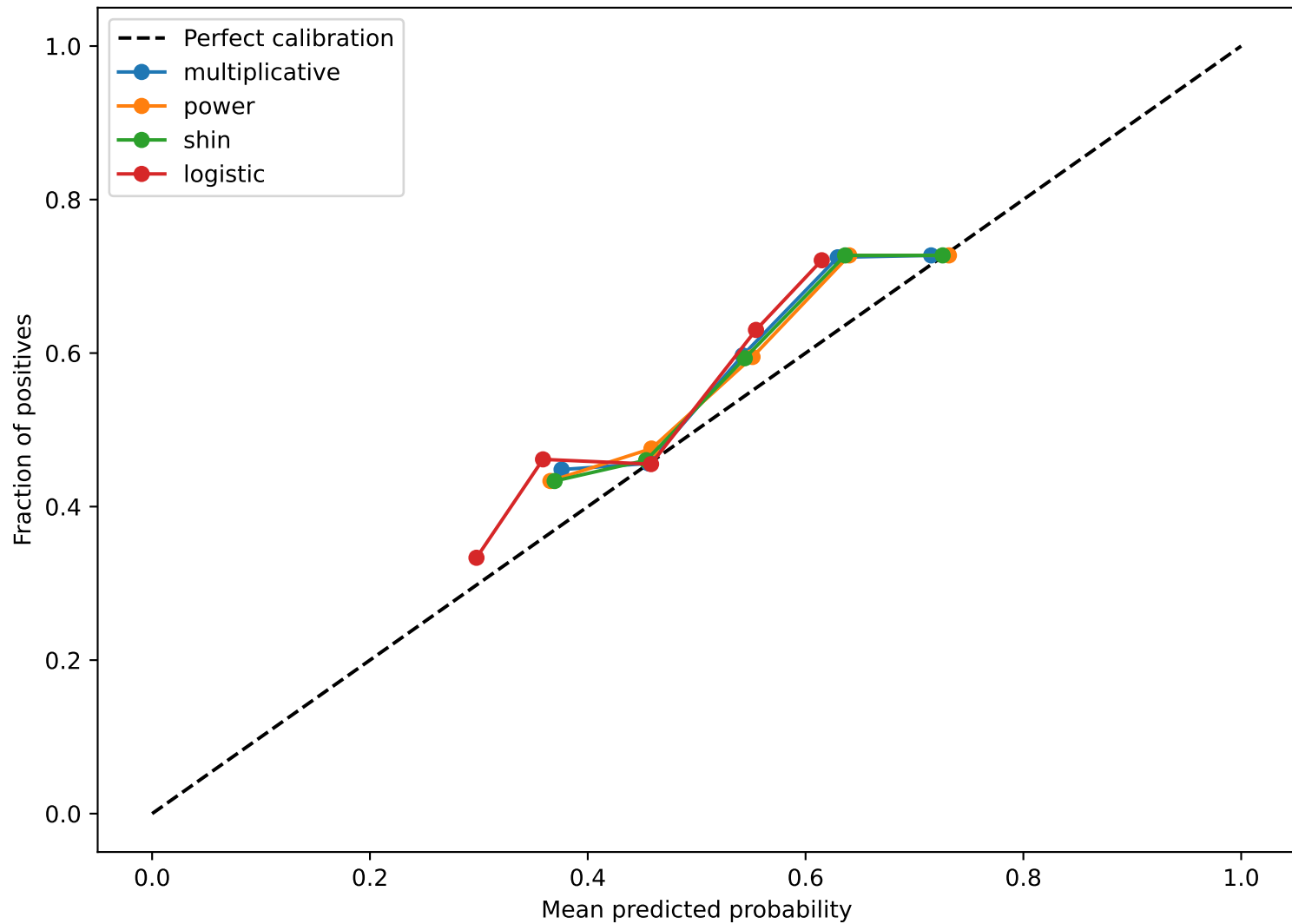
Calibration curves - Over/Under Football
