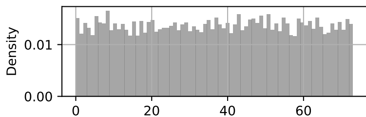
Prior: tau
