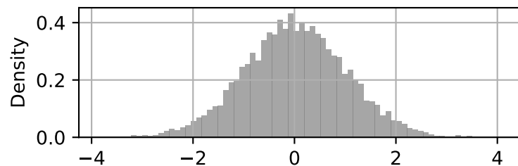
Prior: beta2
