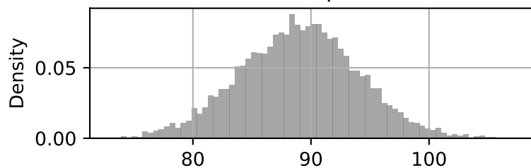
Prior: alpha2
