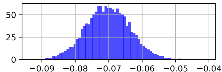
Posterior: beta2
