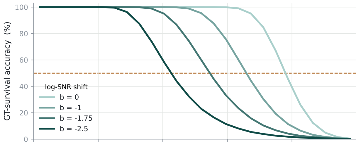
scape_diffusionnet_512_FMD: GT survival vs t (model-free, 50 pairs, 6 draws)
