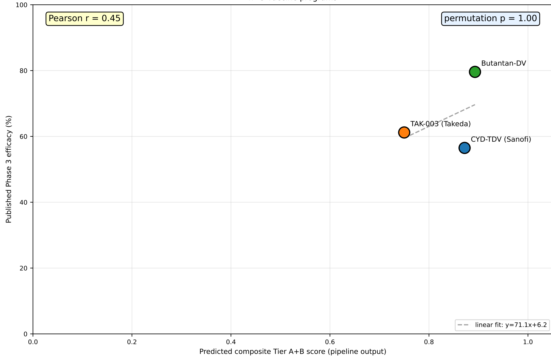
Fig 3. Retrospective Phase 3 validation: predicted composite scores vs published clinical efficacy n=3 vaccine programs
