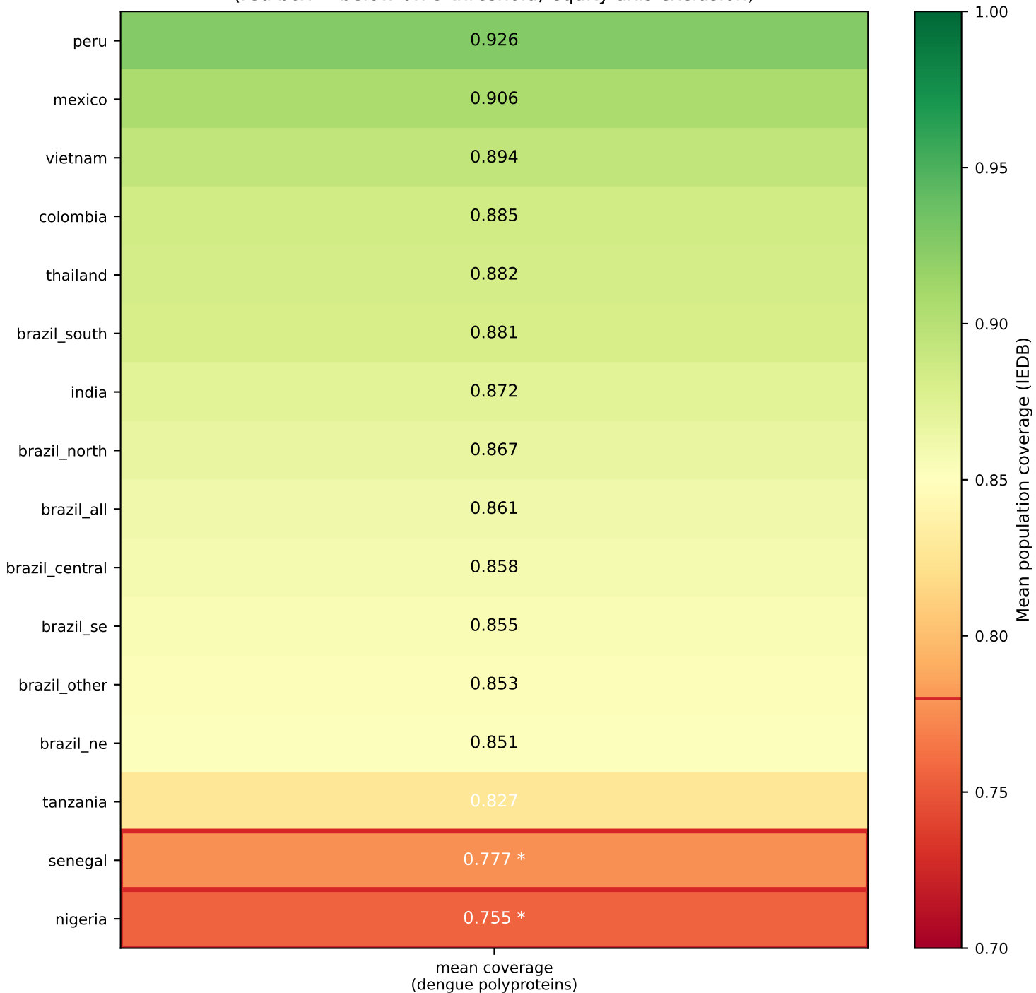
Fig 4. HLA Class I population coverage of DENV-1-4 polyproteins across 16 dengue-endemic regions (red box = below 0.78 threshold; equity axis exclusion)
