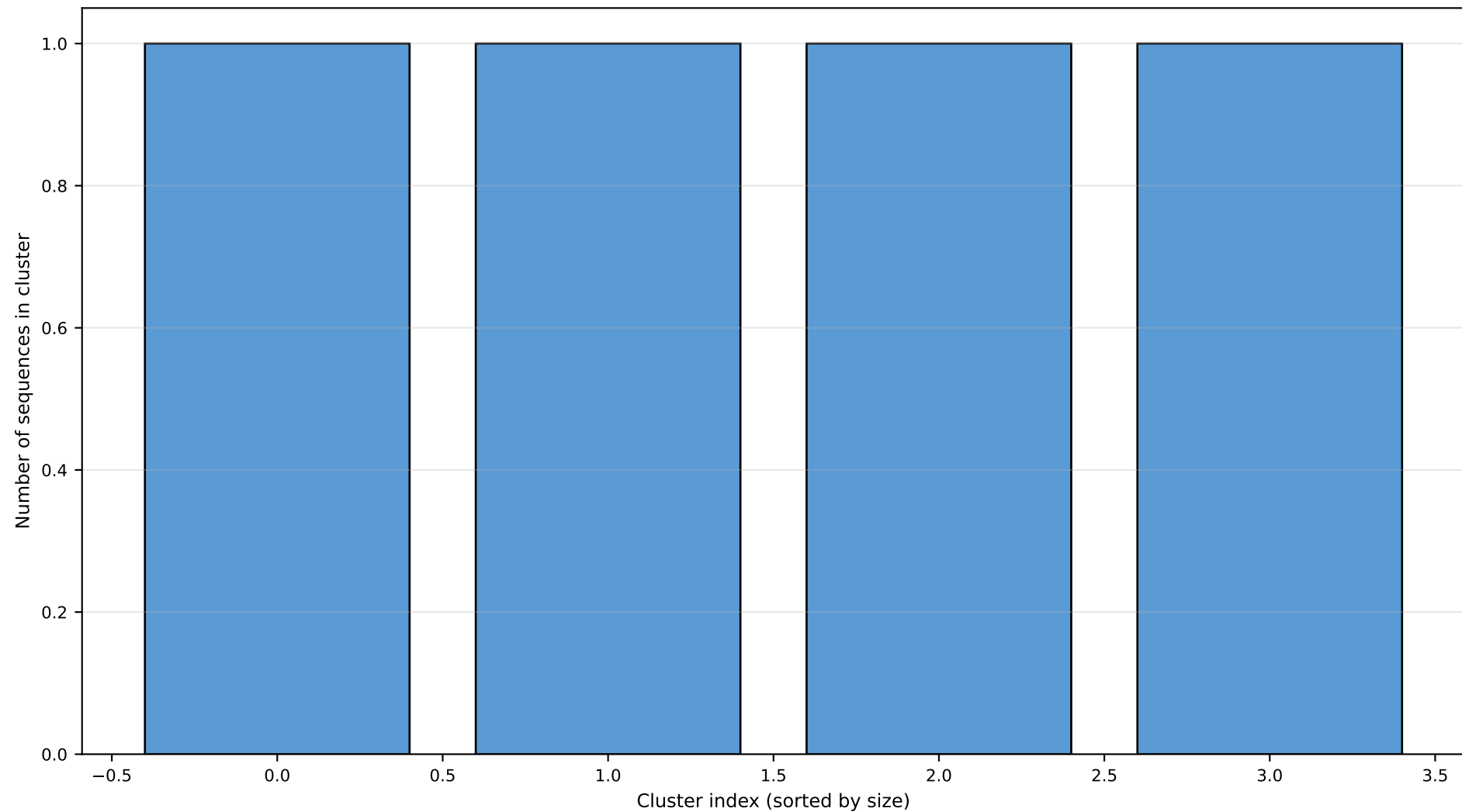
Fig 6. CDHIT redundancy clustering across 4 input sequences (4 non-redundant clusters; centroids feed downstream B-cell + T-cell scoring)
