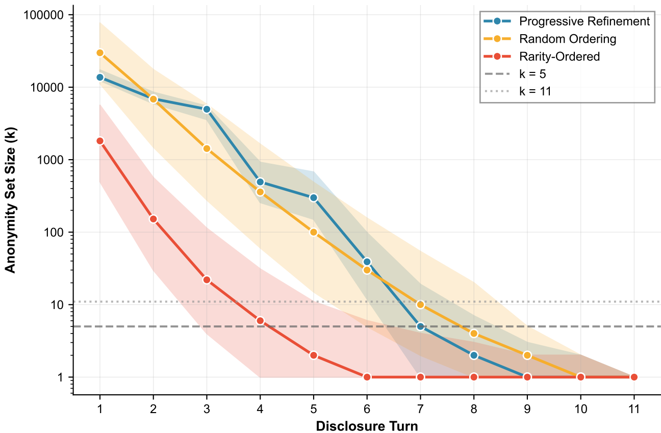
Anonymity Set Size (k) Across Disclosure Turns
