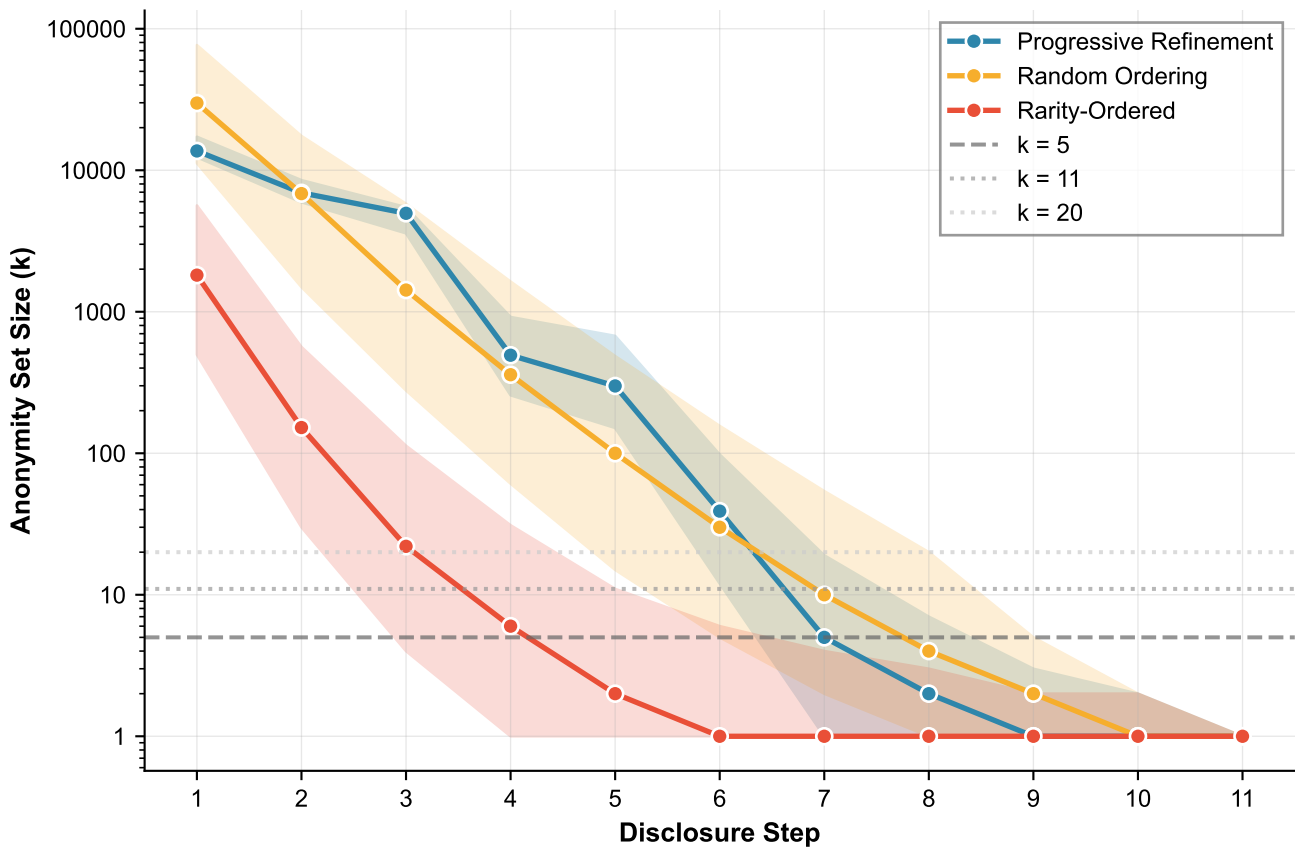
Anonymity Set Size (k) Across Disclosure Steps
