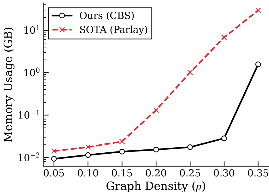
Memory ( N=1000, r=5, s=9 )
