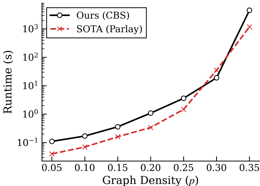
Runtime ( N=1000, r=4, s=8 )
