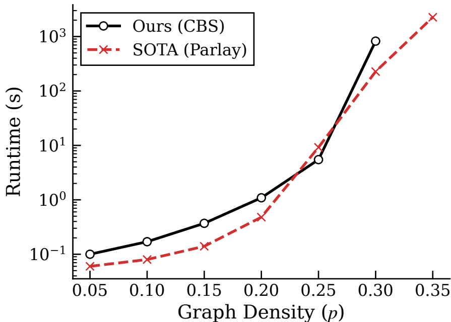
Runtime ( N=1000, r=4, s=7 )
