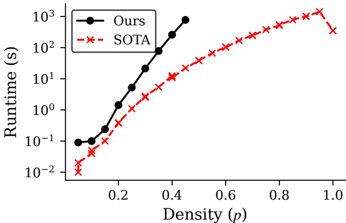
Runtime vs Density ( N=500, r=4, s=5 )
