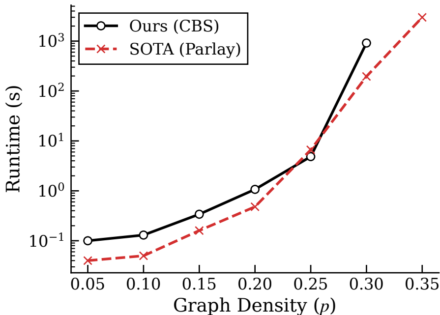
Runtime ( N=1000, r=5, s=7 )
