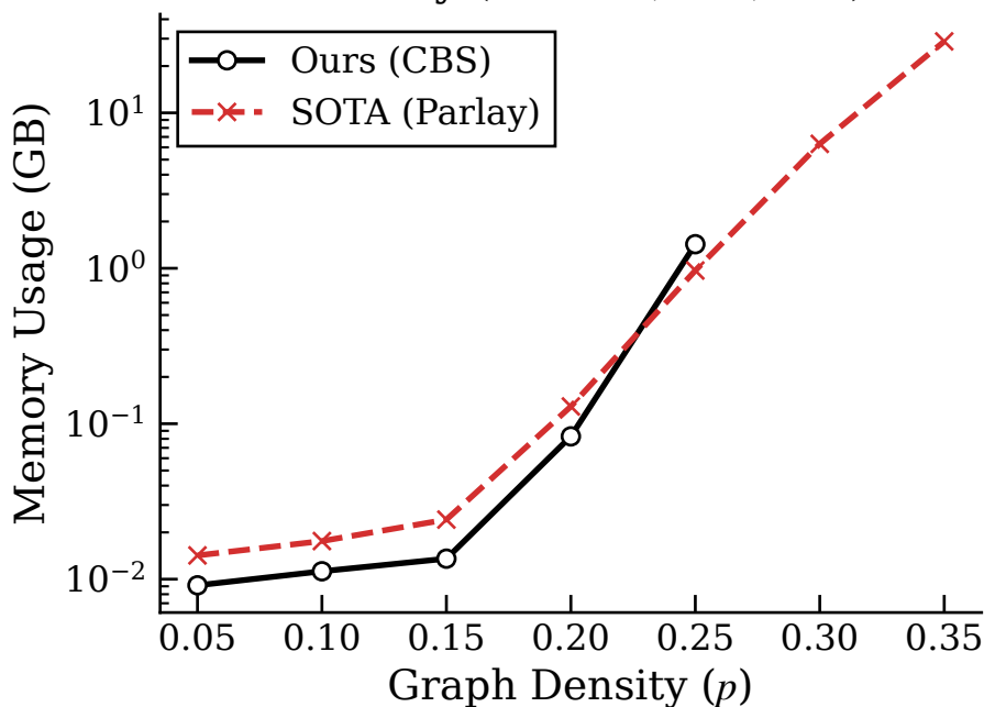
Memory ( N=1000, r=5, s=6 )
