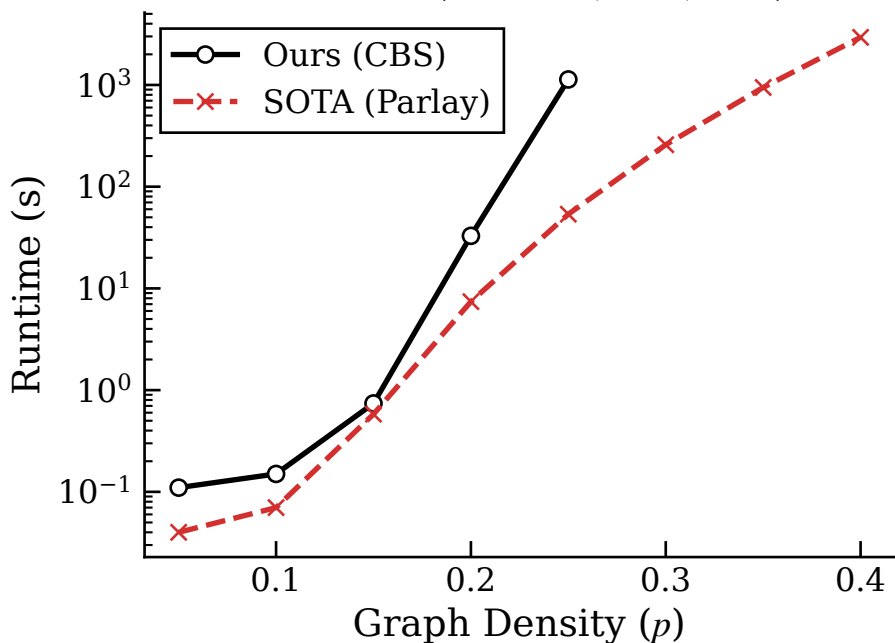
Runtime ( N=1000, r=4, s=5 )
