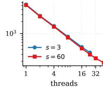
web-Stanford
