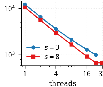
soc-pokec
