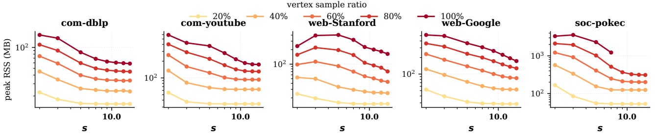
Figure 10: Vertex-induced scalability of SPIN*: peak RSS under the same protocol as Figure 9.
