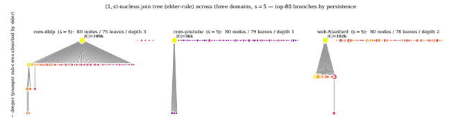
Figure 8: Nucleus join tree at s = 5 across three domains.
