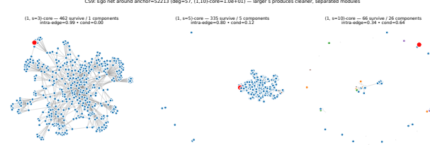
Figure 7: Ego-network around a com-dblp anchor under three s values.
