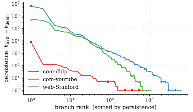
Figure 12: Branch persistence vs. rank at s=5 (log-log): long tail = deep hierarchy.
