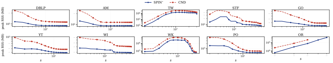
Figure 4: Memory usage across ten graphs.
