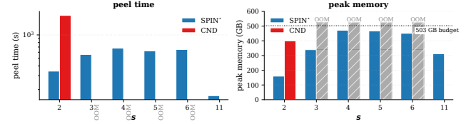
Figure 7: com-friendster (1.806B edges, the largest SNAP graph): SPIN* completes the (1, s) decomposition at every tested s \in \{2, 3, 4, 5, 6, 11\} while CND only completes at s=2 and exceeds the 503 GB budget at every s \geq 3 tested. On the one matched cell, SPIN* peels in 344 s vs. 1,775 s (5.2 \times ) using 160 GB vs. 400 GB (2.5 \times less).
