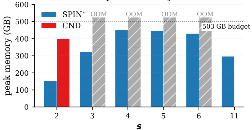
peak memory
