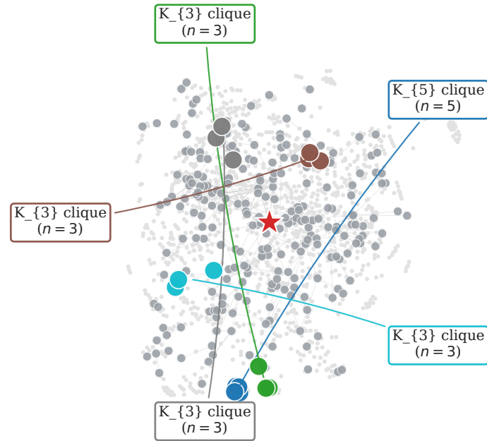
s = 7 : peeled 1199/1452, max clique K_5
