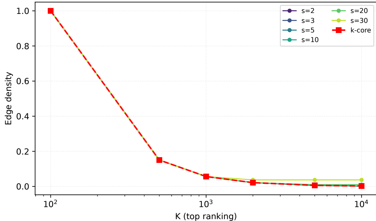
CS3(c): Induced edge density vs K
