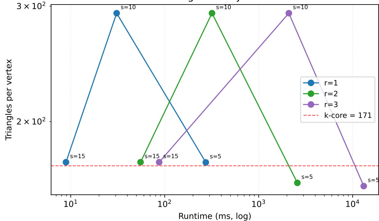
CS7b: Triangle density vs runtime
