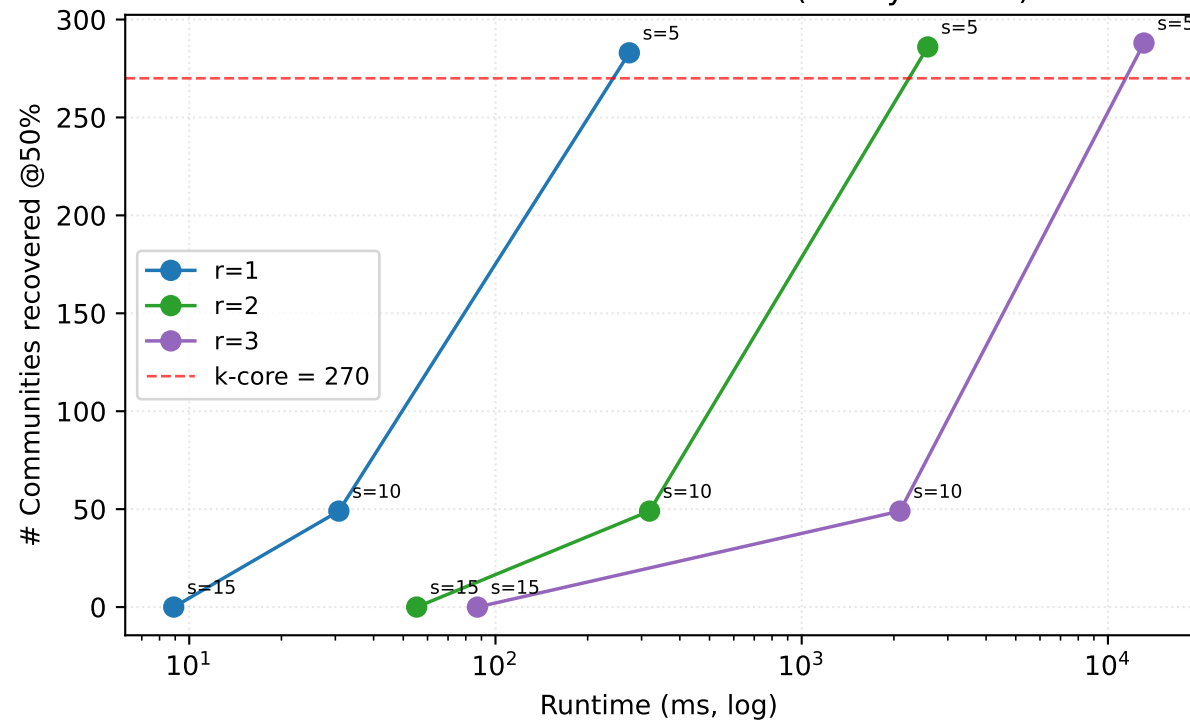
CS7a: Communities vs runtime (com-youtube)
