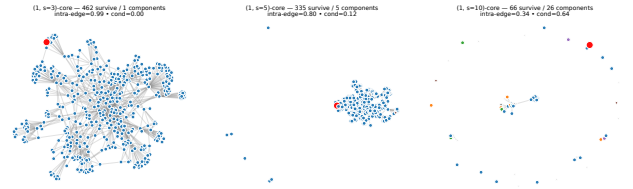
Figure 7: Ego-network around a com-dblp anchor under three s values.
