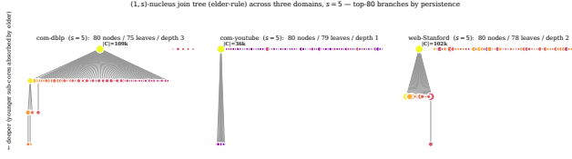
Figure 8: Nucleus join tree at s = 5 across three domains.
