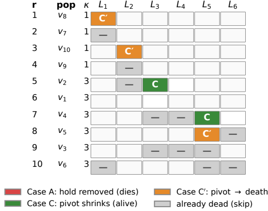
Figure 2: Incremental peel trace on the running example.
