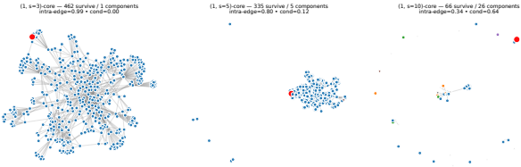
Figure 7: Two-hop ego-network of a com-dblp anchor under (1, s) -decomposition. Vertices are colored by connected component among surviving vertices. Observe that increasing s splits one large local structure into smaller components.
