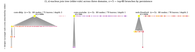
Figure 8: (1, s) -clique-connected nucleus join tree at s = 5 across three domains. Observe that the hierarchy shapes differ across collaboration, social, and web graphs.
