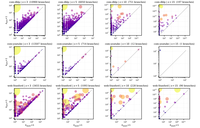
Figure 9: Persistence diagrams across three domains and four s values. Observe that branch persistence changes with both domain and clique size.
