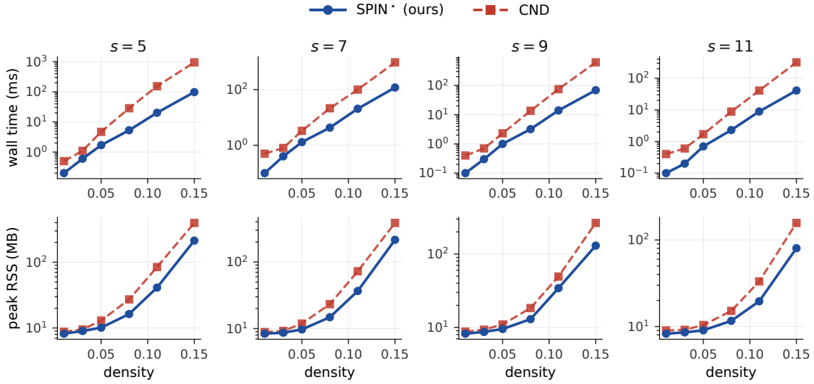
Figure 5: Dense-synthetic stress test.
