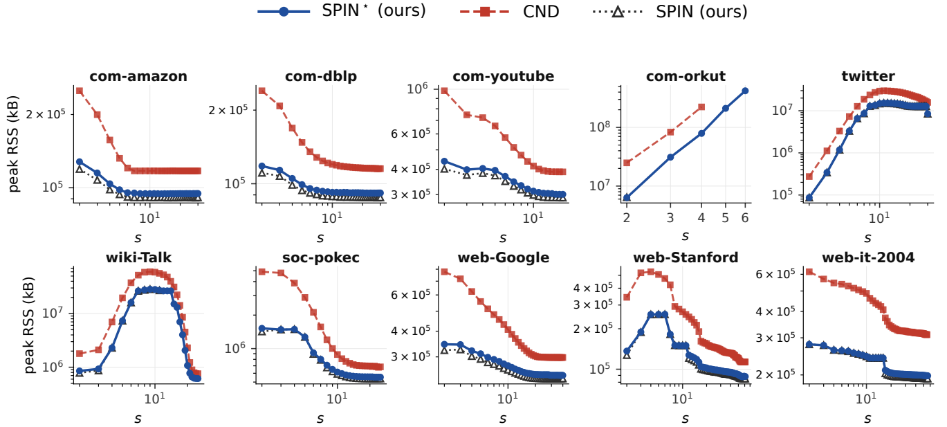
Figure 4: Peak RSS across ten graphs.
