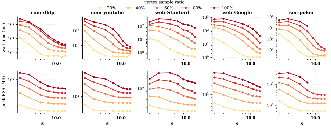
Figure 6: Vertex-induced scalability of SPIN*.
