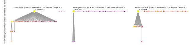
Figure 17: (1, s) -clique-connected nucleus join tree at s = 5 across three domains. Observe that the hierarchy shapes differ across collaboration, social, and web graphs.
