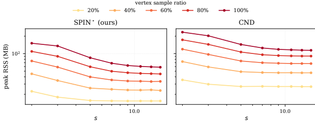
Figure 11: Vertex-induced scalability: peak RSS under the same protocol as Figure 10.
