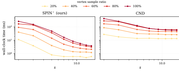
Figure 10: Vertex-induced scalability: wall-clock time of SPIN* (left) and CND (right) as s varies, with one curve per vertex-sample ratio. Higher ratios consistently take longer; the curves do not cross.
