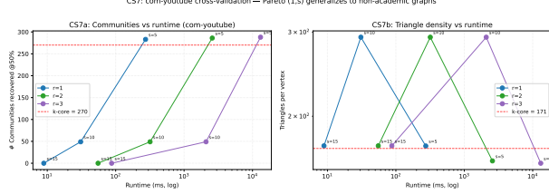
Figure 15: Quality-runtime Pareto plot on com-youtube for r \in \{1, 2, 3\} and s \in \{5, 10, 15\} . Observe that r = 1 reaches the same quality contours as higher- r settings with lower runtime.
