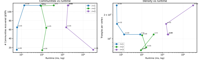
Figure 14: Quality-runtime Pareto plot on com-dblp for r \in \{1, 2, 3\} and s \in \{5, 10, 15, 20\} . Observe that the r = 1 points lie on the favorable quality-runtime frontier in the DBLP settings.
