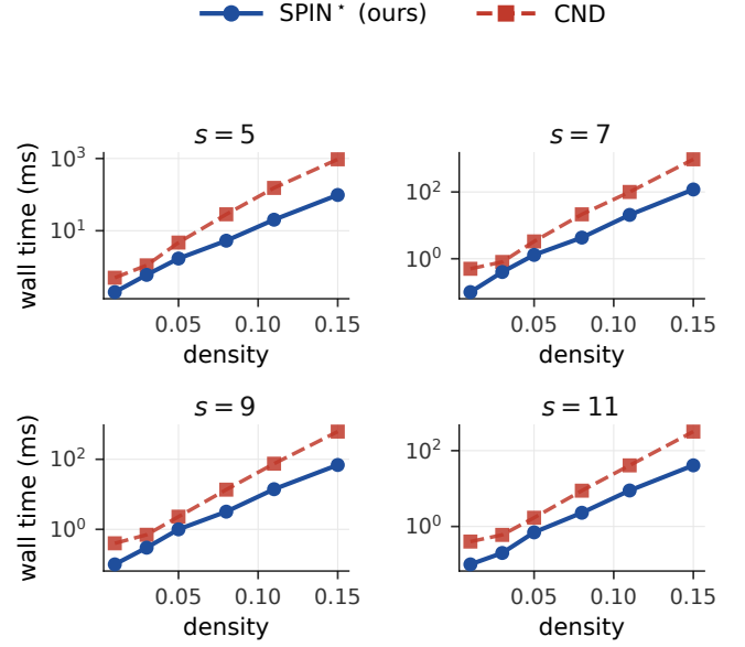
Figure 5: Runtime stress test on synthetic clique-injection graphs with |V| = 1000 . Solid blue is SPIN*, and dashed red is CND. Runtime grows rapidly as density and s increase.
