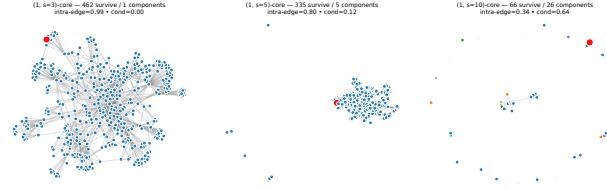
Figure 11: Two-hop ego-network of a com-dblp anchor under (1, s) -decomposition. Vertices are colored by connected component among surviving vertices. Observe that increasing s splits one large local structure into smaller components.
