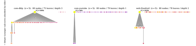
Figure 12: (1, s) -clique-connected nucleus join tree at s = 5 across three domains. Observe that the hierarchy shapes differ across collaboration, social, and web graphs.
