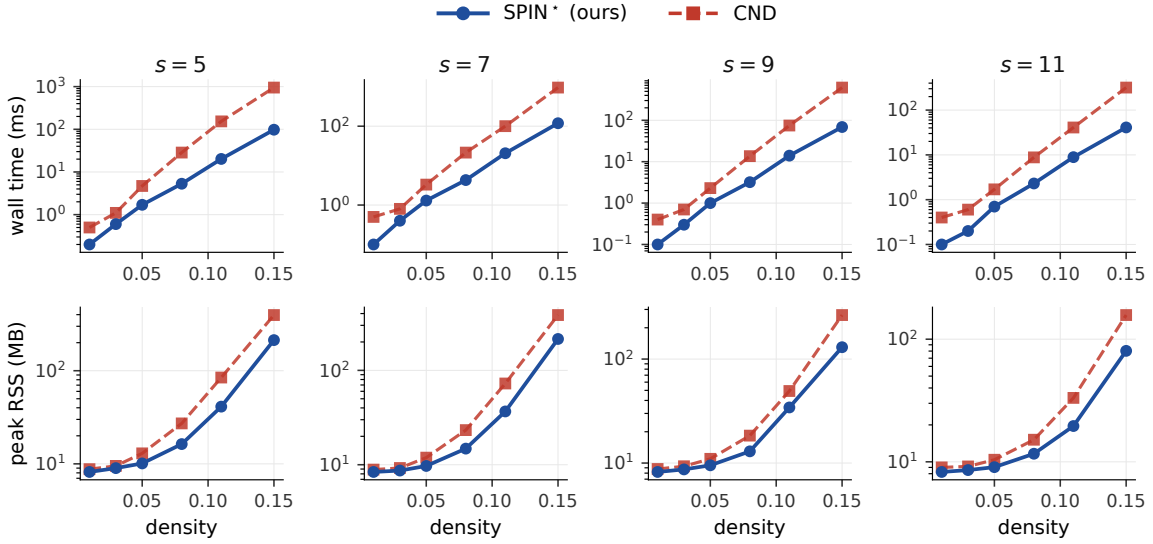
Figure 5: Synthetic clique-injection stress test on |V|=1000 graphs. Solid blue is SPIN*, dashed red is CND. Top row: wall time grows rapidly with density and s . Bottom row: peak RSS under the same protocol; the memory gap widens as mutable residual state amplifies dense-clique growth.
