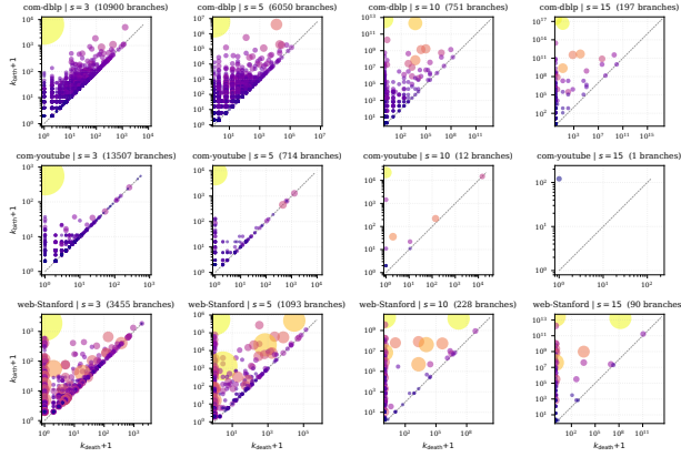
Figure 13: Persistence diagrams across three domains and four s values. Observe that branch persistence changes with both domain and clique size.
