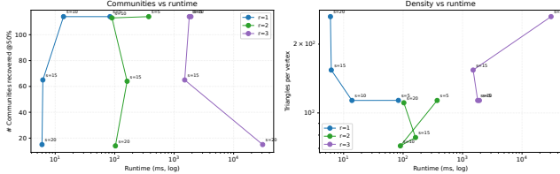
Figure 9: Quality-runtime Pareto plot on com-dblp for r \in \{1, 2, 3\} and s \in \{5, 10, 15, 20\} . Observe that the r = 1 points lie on the favorable quality-runtime frontier in the DBLP settings.
