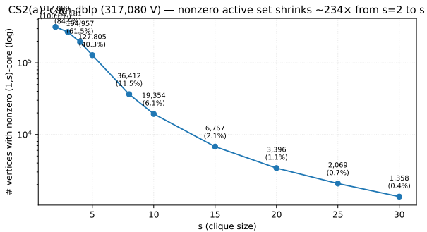
Figure 8: Active-set size on com-dblp as s varies. Observe that larger s sharply shrinks the vertices with nonzero (1, s) -core value.
