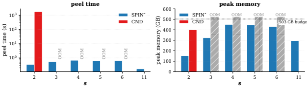
Figure 7: com-friendster (1.806B edges): peel time (left) and peak memory (right). CND completes only at s=2 ; for s \geq 3 it exceeds the 503 GB budget.
