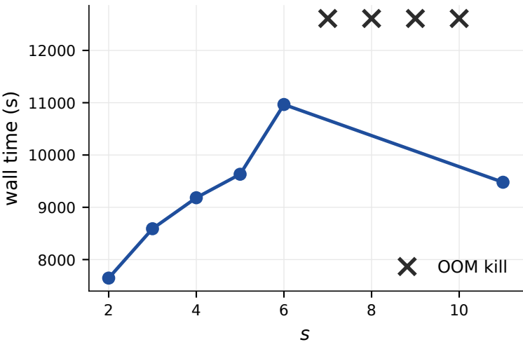
com-friendster, |E| = 1.8B , T = 24
