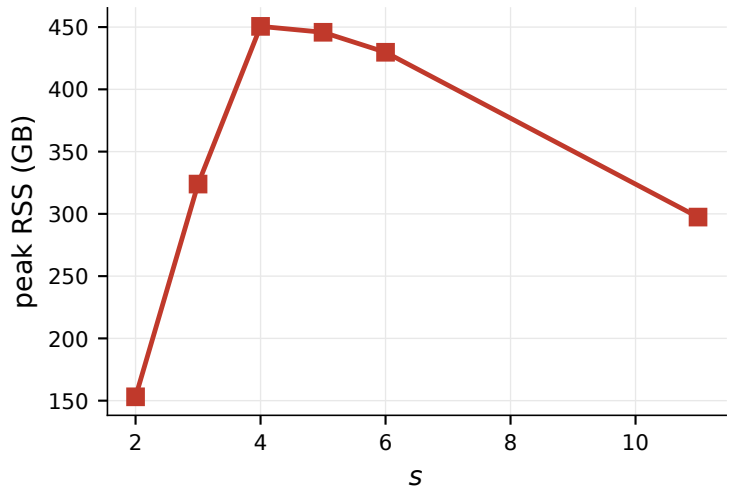
com-friendster peak memory
