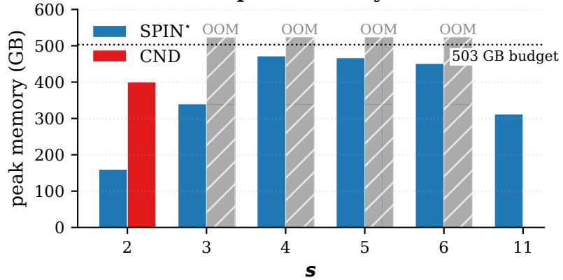
peak memory
