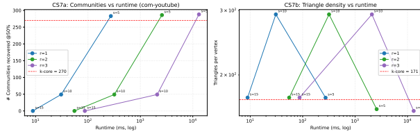
Figure 15: Quality-runtime Pareto plot on com-youtube for r \in \{1, 2, 3\} and s \in \{5, 10, 15\} . Observe that r = 1 reaches the same quality contours as higher- r settings with lower runtime.
