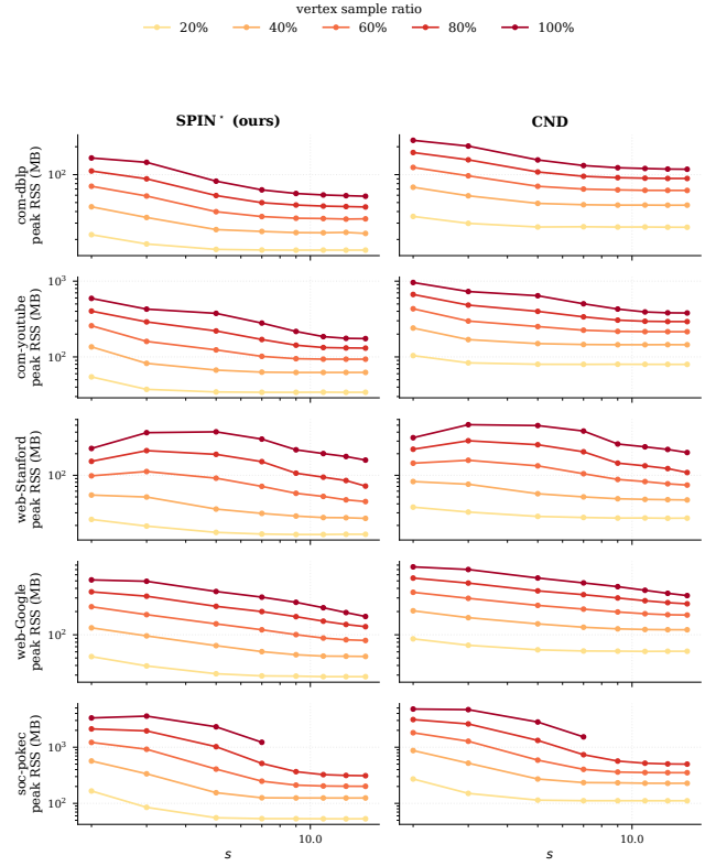
Figure 11: Vertex-induced scalability: peak RSS under the same protocol as Figure 10.
