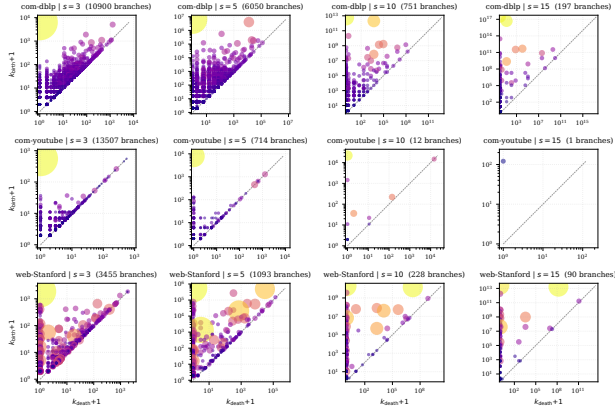
Figure 18: Persistence diagrams across three domains and four s values. Observe that branch persistence changes with both domain and clique size.
