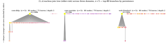
Figure 15: (1, s) -clique-connected nucleus join tree at s = 5 across three domains. Observe that the hierarchy shapes differ across collaboration, social, and web graphs.
