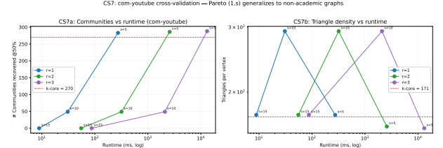
Figure 13: Quality-runtime Pareto plot on com-youtube for r \in \{1, 2, 3\} and s \in \{5, 10, 15\} . Observe that r = 1 reaches the same quality contours as higher- r settings with lower runtime.
