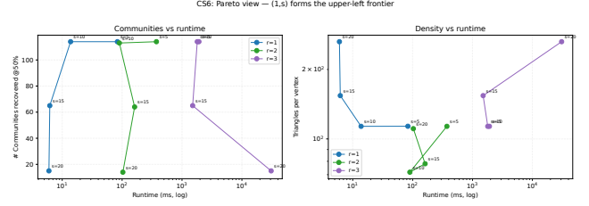
Figure 12: Quality-runtime Pareto plot on com-dblp for r \in \{1, 2, 3\} and s \in \{5, 10, 15, 20\} . Observe that the r = 1 points lie on the favorable quality-runtime frontier in the DBLP settings.
