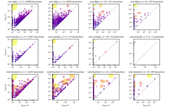
Figure 16: Persistence diagrams across three domains and four s values. Observe that branch persistence changes with both domain and clique size.
