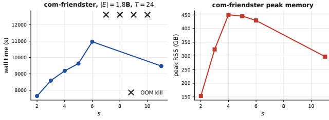
Figure 7: SPIN* on com-friendster (1.806B edges) at T=24 : wall time (left) and peak RSS (right) as s varies. Crosses mark the s values where construction hit the 503 GB cap and the kernel killed the process. SPIN* peels the static CPI in under one second on every successful configuration; construction dominates wall time at this scale.
