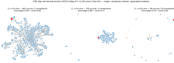
Figure 14: Two-hop ego-network of a com-dblp anchor under (1, s) -decomposition. Vertices are colored by connected component among surviving vertices. Observe that increasing s splits one large local structure into smaller components.
