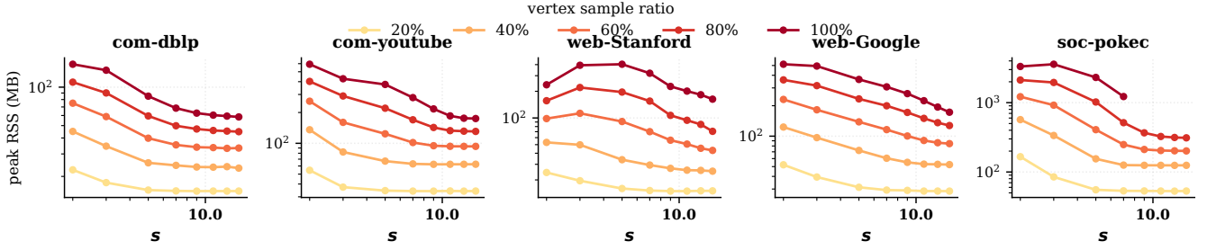
Figure 9: Vertex-induced scalability of SPIN*: peak RSS under the same protocol as Figure 8.
