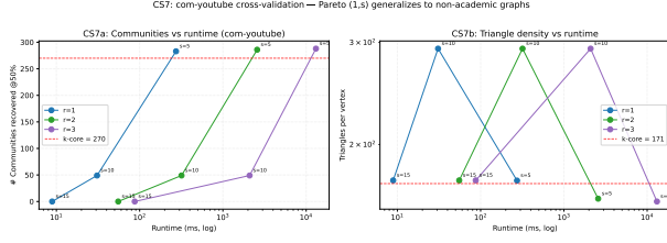
Figure 13: Quality-runtime Pareto plot on com-youtube for r \in \{1, 2, 3\} and s \in \{5, 10, 15\} . Observe that r = 1 reaches the same quality contours as higher- r settings with lower runtime.
