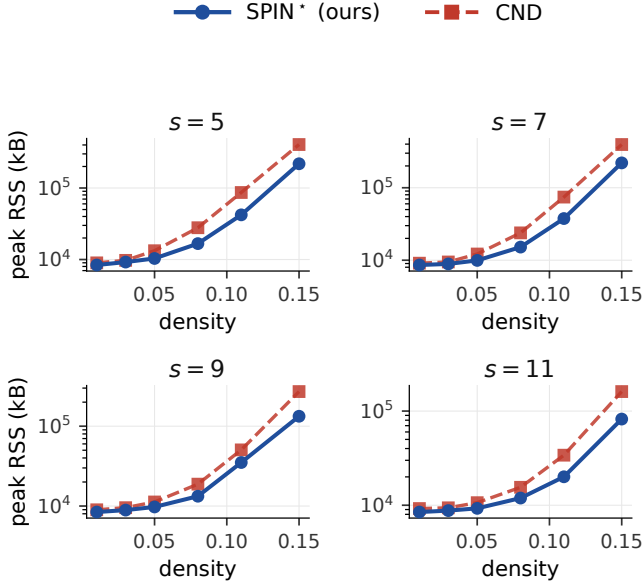
Figure 6: Peak resident-set memory under the same stress-test protocol as Figure 5. The memory gap shows when mutable residual state amplifies dense-clique growth.
