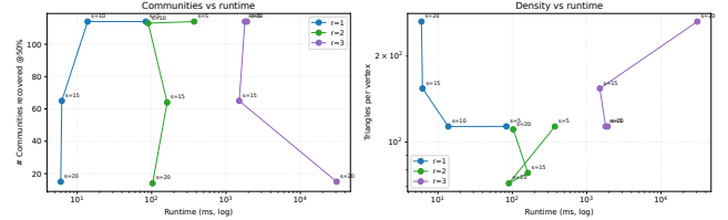
Figure 12: Quality-runtime Pareto plot on com-dblp for r \in \{1, 2, 3\} and s \in \{5, 10, 15, 20\} . Observe that the r = 1 points lie on the favorable quality-runtime frontier in the DBLP settings.
