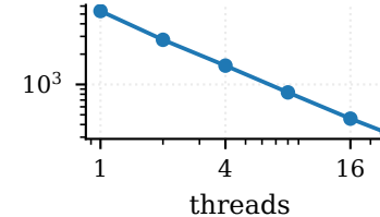
web-Stanford
