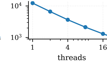
soc-pokec
