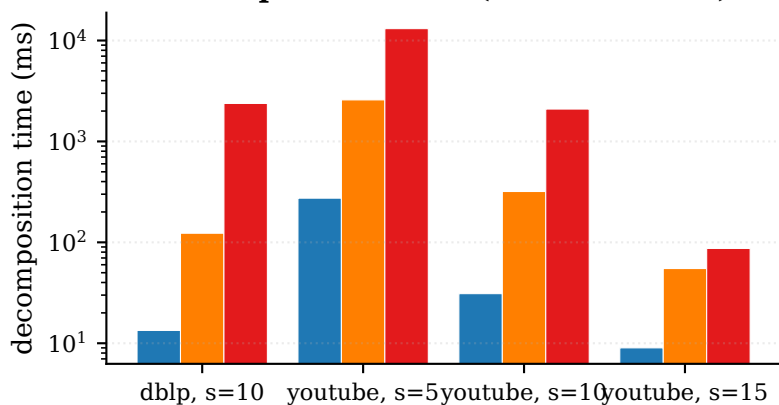
decomposition time (lower is better)
