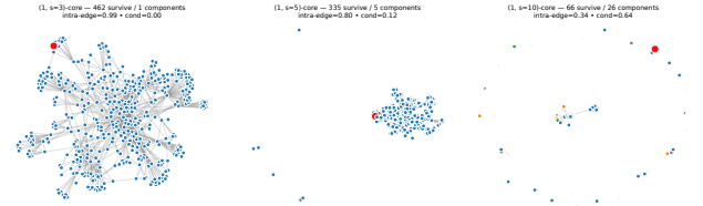
Figure 14: Two-hop ego-network of a com-dblp anchor under (1, s) -decomposition. Vertices are colored by connected component among surviving vertices. Observe that increasing s splits one large local structure into smaller components.
