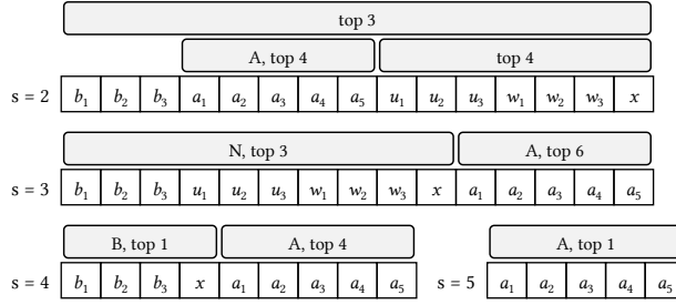
Figure 2: One hierarchy per size (STrees) for Figure 1: for every size, its tree drawn over the depth-first array of its vertices; a node is a bar over the vertices it contains.
