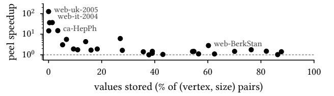
Figure 6: Peel speedup from the settled vertices.
