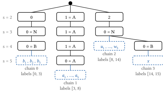
Figure 4: The trie that refines the chains of Figure 1 size by size; the vertices stop at the dashed leaves.
