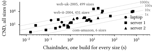
Figure 5: Build time of CND, all sizes, against ChainIndex.
