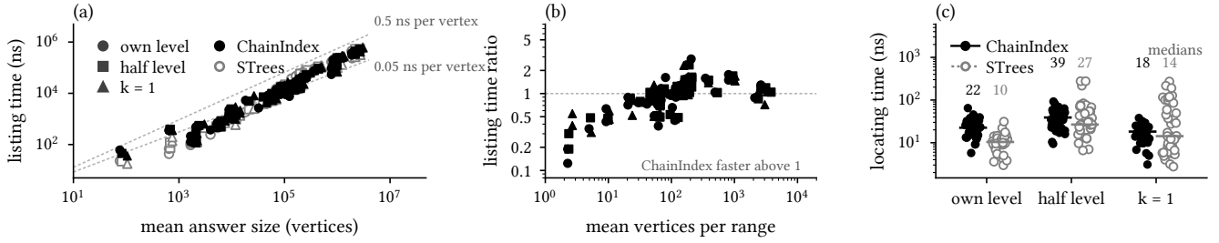
Figure 7: Community queries: (a) listing time by answer size and level, (b) listing time of STrees over that of ChainIndex by vertices per range, (c) locating time by level.
