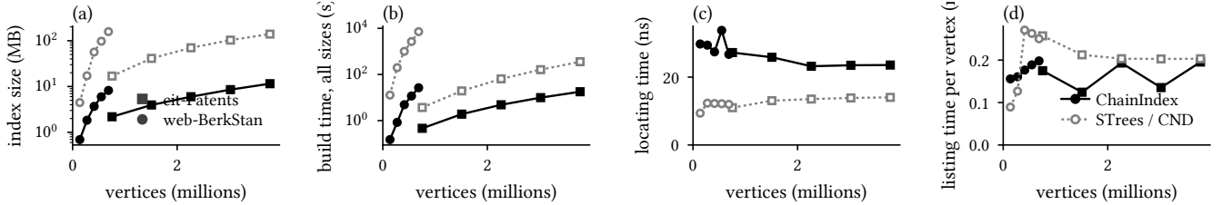
Figure 9: Scalability over vertex-induced samples.
