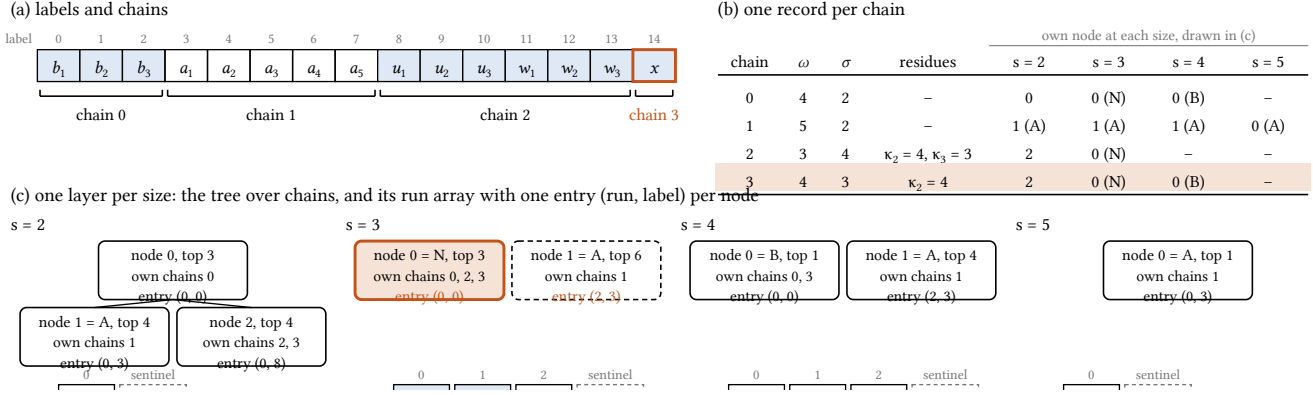
Figure 3: ChainIndex for Figure 1: (a) the labels and the four chains, (b) the record of every chain, (c) the layer of every size, and the community query of x at (3, 2) traced through them (Example 6.1).
