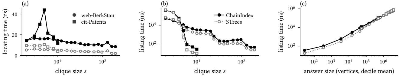
Figure 8: Own-level latency by clique size and by answer size.
