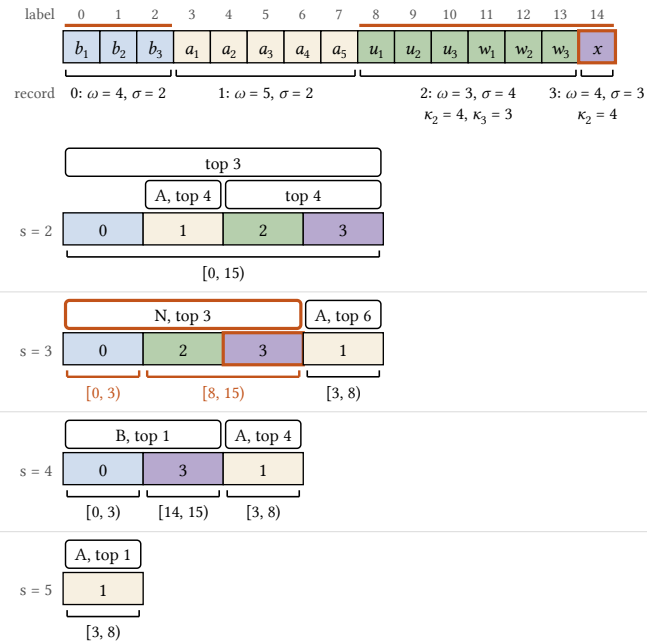
(b) ChainIndex
