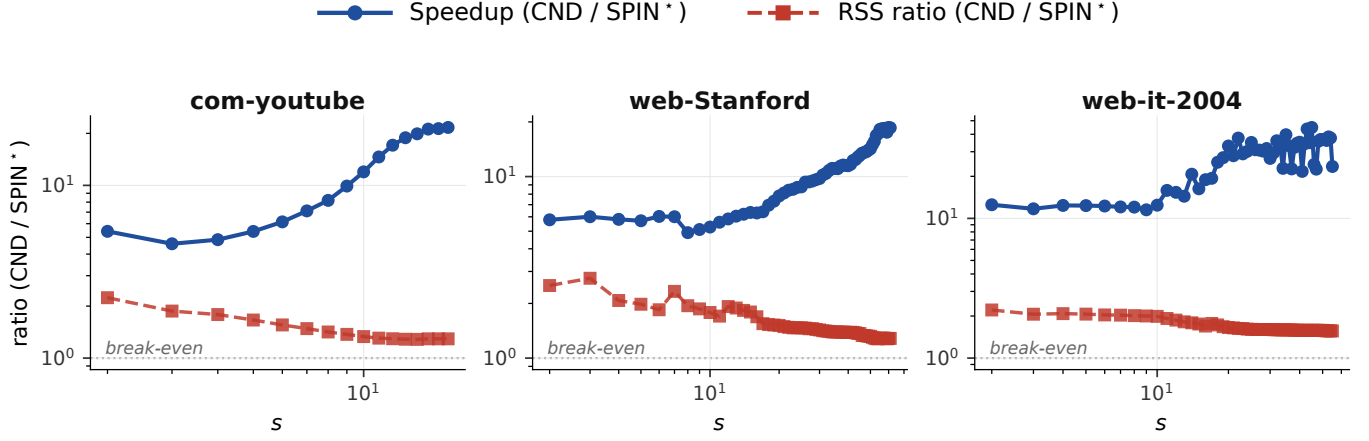
Figure 6: Speedup and peak-RSS ratio on com-youtube, web-Stanford, and web-it-2004. The curves show CND divided by SPIN* on matched successful configurations. Values above 1 mean SPIN* is faster or uses less memory.
