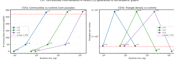
Figure 14: Quality-runtime Pareto plot on com-youtube for r \in \{1, 2, 3\} and s \in \{5, 10, 15\} . Observe that r = 1 reaches the same quality contours as higher- r settings with lower runtime.
