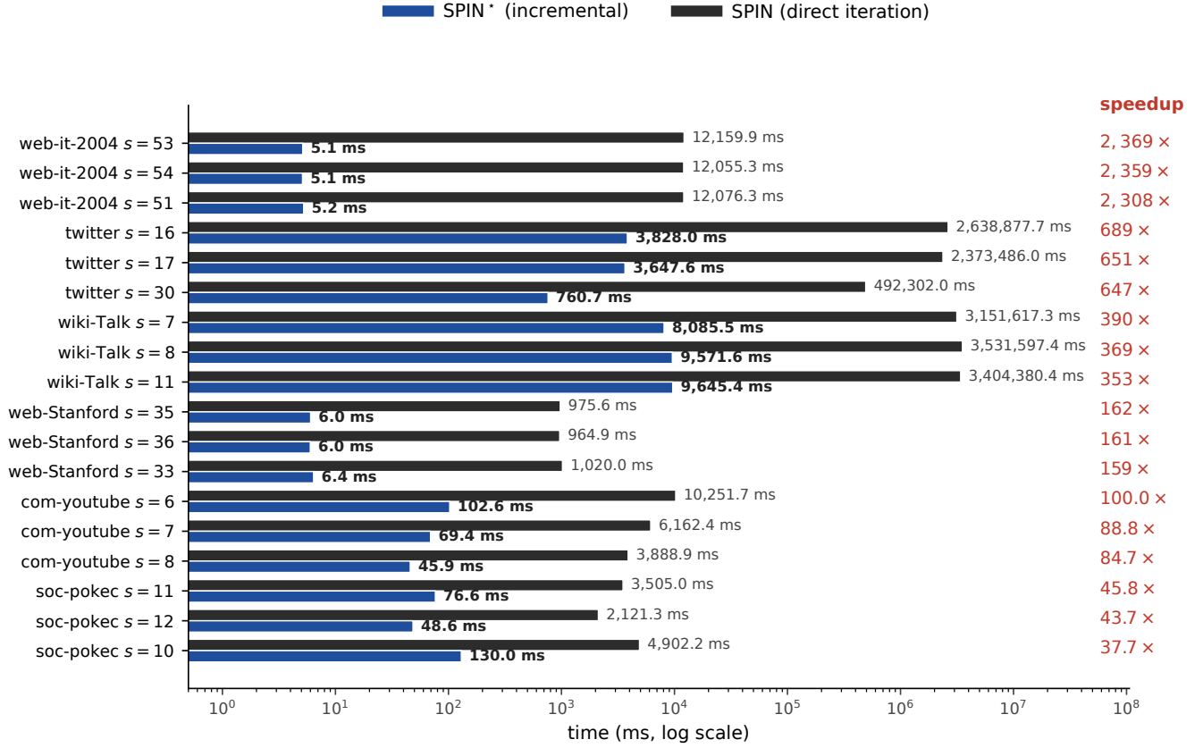
Figure 7: Per-cell wall-clock time of SPIN* (incremental) versus SPIN (direct iteration), showing the top three matched ( graph, s ) cells by speedup for each of the six graphs where the gap is largest. Both algorithms compute the same (1, s) -core values; SPIN* avoids redundant full-graph passes by only revisiting vertices whose path counters changed.
