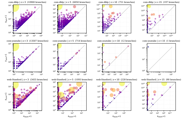
Figure 17: Persistence diagrams across three domains and four s values. Observe that branch persistence changes with both domain and clique size.
