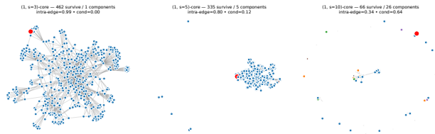
Figure 15: Two-hop ego-network of a com-dblp anchor under (1, s) -decomposition. Vertices are colored by connected component among surviving vertices. Observe that increasing s splits one large local structure into smaller components.
