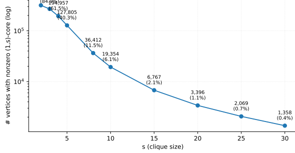
Figure 11: Active-set size on com-dblp as s varies. Observe that larger s sharply shrinks the vertices with nonzero (1, s) -core value.
