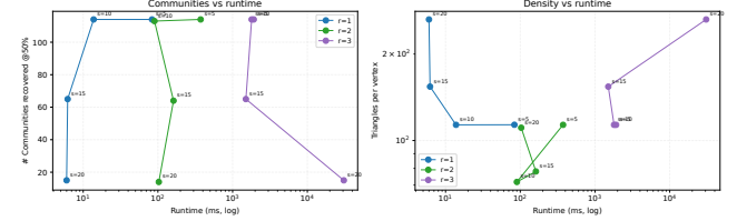
Figure 13: Quality-runtime Pareto plot on com-dblp for r \in \{1, 2, 3\} and s \in \{5, 10, 15, 20\} . Observe that the r = 1 points lie on the favorable quality-runtime frontier in the DBLP settings.
