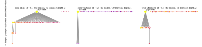
Figure 16: (1, s) -clique-connected nucleus join tree at s = 5 across three domains. Observe that the hierarchy shapes differ across collaboration, social, and web graphs.
