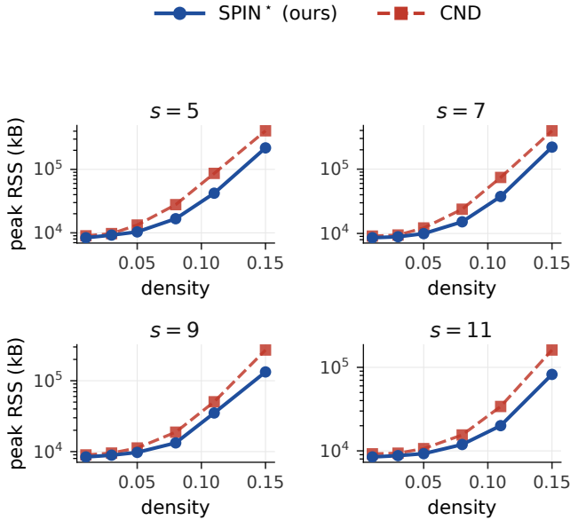
Figure 9: Peak resident-set memory under the same stress-test protocol as Figure 8. The memory gap shows when mutable residual state amplifies dense-clique growth.
