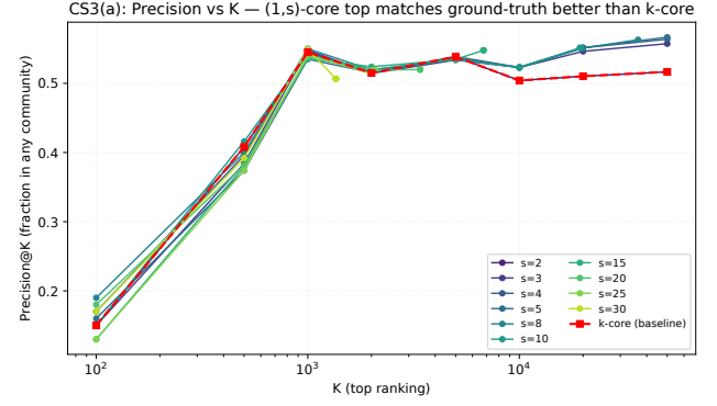
Figure 12: Precision@ K on com-dblp. Observe that the (1, s) -core rankings for s \in \{3, 5, 10, 15\} stay above the k -core curve in the plotted range.
