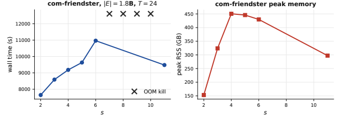
Figure 10: SPIN* on com-friendster (1.806B edges) at T=24 : wall time (left) and peak RSS (right) as s varies. Crosses mark the s values where construction hit the 503 GB cap and the kernel killed the process. SPIN* peels the static CPI in under one second on every successful configuration; construction dominates wall time at this scale.
