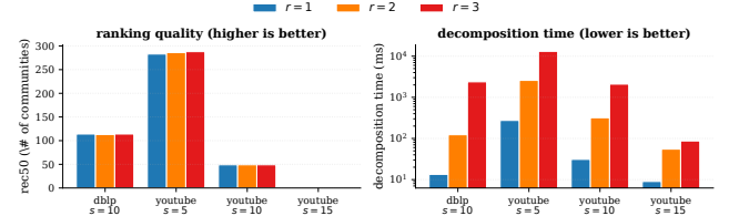
Figure 10: Cross- r comparison on com-dblp ( s=10 ) and com-youtube ( s \in \{5, 10, 15\} ). Left: ranking quality (rec50, higher is better) is nearly identical across r . Right: decomposition time (log scale, lower is better) is 1–3 orders of magnitude smaller at r=1 .
