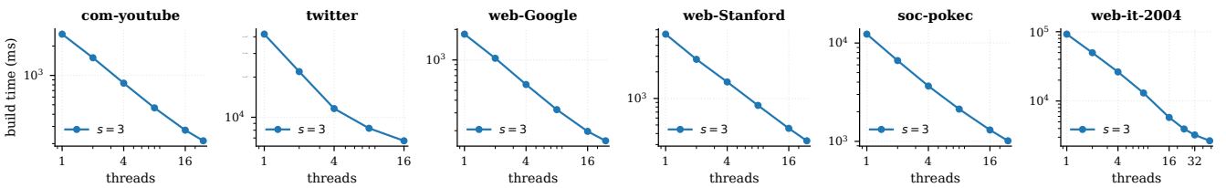
Figure 6: ParaBuild build time vs. thread count; one curve per representative s , ending at its optimum T .
