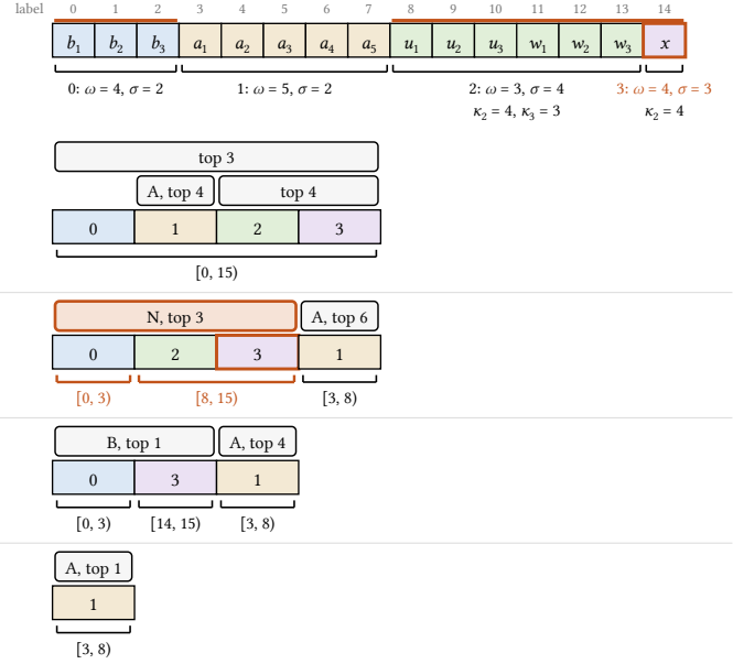
Figure 2: Baseline (a) and ChainIndex (b) for Figure 1, one row per size; the query of x at (3, 2) in orange.
