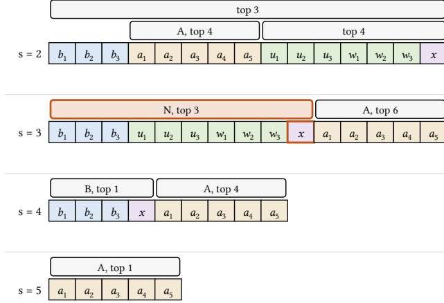
Figure 2: Baseline (a) and ChainIndex (b) for Figure 1, one row per size; the query of x at (3, 2) in orange.
