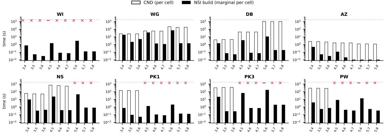
Figure 2: Build time per grid cell (log scale).
