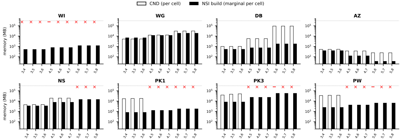
Figure 3: Build memory per grid cell (log scale).
