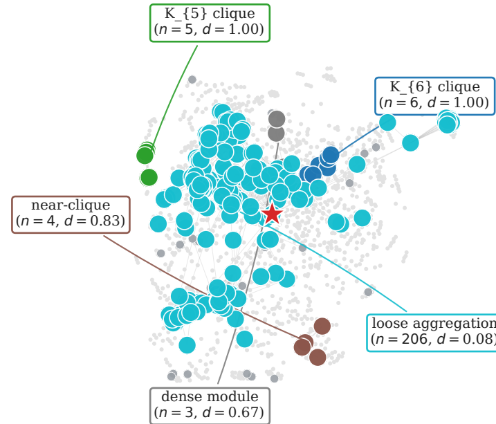
s = 10 : peeled 1204/1452, max clique K_6
