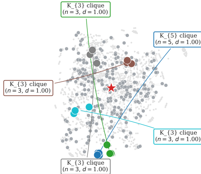
s = 7 : peeled 1199/1452, max clique K_5
