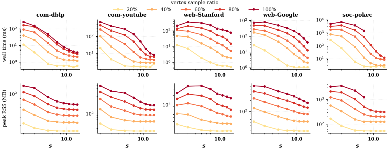
Figure 6: Vertex-induced scalability: wall time (top) and peak RSS (bottom).
