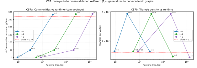
Figure 11: Quality-runtime Pareto plot on com-youtube for r \in \{1, 2, 3\} and s \in \{5, 10, 15\} . Observe that r = 1 reaches the same quality contours as higher- r settings with lower runtime.
