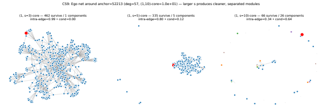
Figure 12: Two-hop ego-network of a com-dblp anchor under (1, s) -decomposition. Vertices are colored by connected component among surviving vertices. Observe that increasing s splits one large local structure into smaller components.
