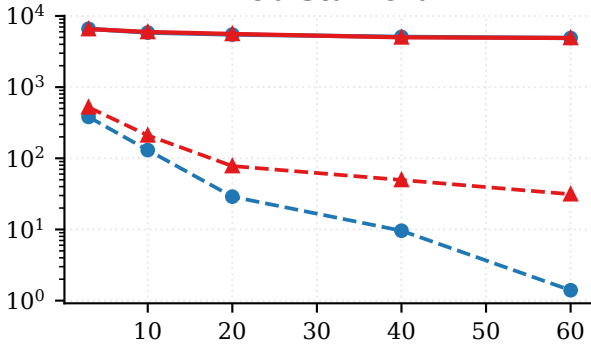
web-Stanford
