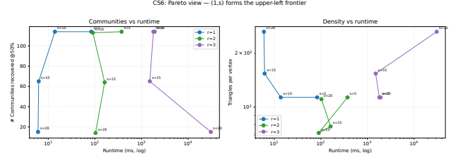
Figure 14: Quality-runtime Pareto plot on com-dblp for r \in \{1, 2, 3\} and s \in \{5, 10, 15, 20\} . Observe that the r = 1 points lie on the favorable quality-runtime frontier in the DBLP settings.
