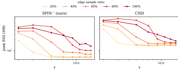
Figure 11: Edge-subsampling scalability: peak RSS under the same protocol as Figure 10.
