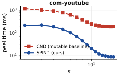
Figure 1: Peel time on com-youtube: SPIN* (ours) versus the mutable-CPI baseline CND as s varies. On this graph alone, SPIN* achieves a 10.6× geometric-mean speedup.
