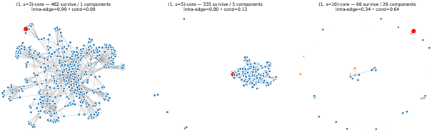
Figure 16: Two-hop ego-network of a com-dblp anchor under (1, s) -decomposition. Vertices are colored by connected component among surviving vertices. Observe that increasing s splits one large local structure into smaller components.
