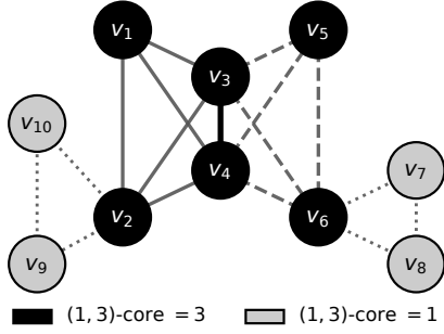
Figure 2: Running example at s = 3 : two K_4 blocks share edge (v_3, v_4) (heavy black); pendant triangles attach at v_2 and v_6 (dotted edges). Black nodes have (1, 3) -core value 3; light-gray nodes have value 1. Edge styles distinguish the two K_4 blocks (solid vs. dashed) from the pendant triangles (dotted).
