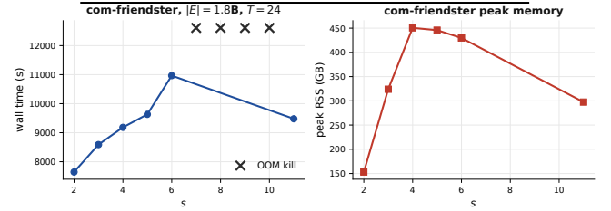
Figure 9: SPIN* on com-friendster (1.806B edges) at T=24 : wall time (left) and peak RSS (right) as s varies. Crosses mark the s values where construction hit the 503 GB cap and the kernel killed the process. SPIN* peels the static CPI in under one second on every successful configuration; construction dominates wall time at this scale.
