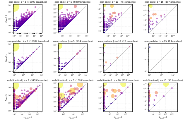
Figure 18: Persistence diagrams across three domains and four s values. Observe that branch persistence changes with both domain and clique size.
