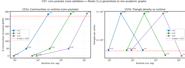
Figure 15: Quality-runtime Pareto plot on com-youtube for r \in \{1, 2, 3\} and s \in \{5, 10, 15\} . Observe that r = 1 reaches the same quality contours as higher- r settings with lower runtime.
