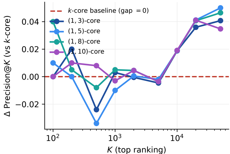
Gain over k -core baseline
