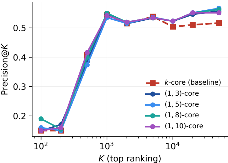
Absolute Precision@K
