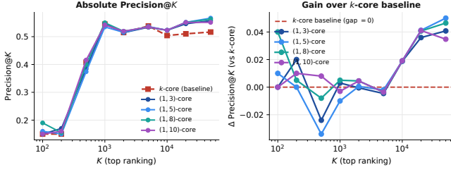
Figure 9: Ground-truth ranking quality on com-dblp. Left: absolute Precision@K — the (1, s)-cores sit above the k-core baseline at large K. Right: gain over the k-core baseline ( y=0 line); (1, s)-cores improve Precision by up to +5 percentage points at K=5 \times 10^4 .
