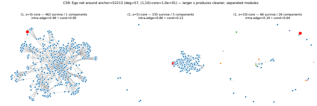
Figure 12: Two-hop ego-network of a com-dblp anchor under (1, s)-decomposition. Vertices are colored by connected component among surviving vertices. Observe that increasing s splits one large local structure into smaller components.
