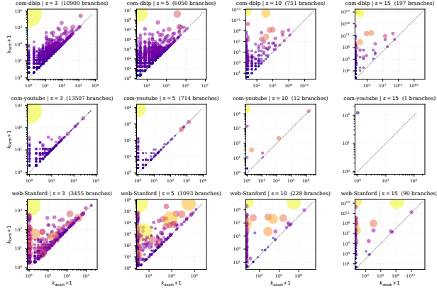
Figure 14: Persistence diagrams across three domains and four s values. Observe that branch persistence changes with both domain and clique size.
