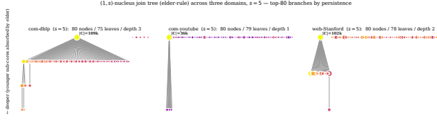
Figure 13: (1, s) -clique-connected nucleus join tree at s = 5 across three domains. Observe that the hierarchy shapes differ across collaboration, social, and web graphs.
