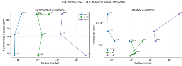
Figure 10: Quality-runtime Pareto plot on com-dblp for r \in \{1, 2, 3\} and s \in \{5, 10, 15, 20\} . Observe that the r = 1 points lie on the favorable quality-runtime frontier in the DBLP settings.
