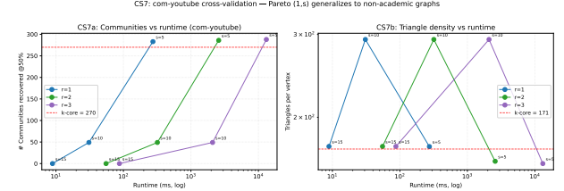
Figure 11: Quality-runtime Pareto plot on com-youtube for r \in \{1, 2, 3\} and s \in \{5, 10, 15\} . Observe that r = 1 reaches the same quality contours as higher- r settings with lower runtime.
