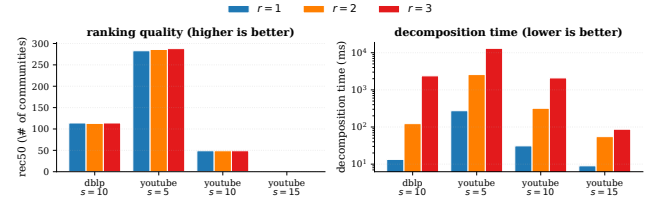
Figure 10: Cross-r comparison on com-dblp (s=10) and com-youtube (s ∈ {5, 10, 15}). Left: ranking quality (rec50, higher is better) is nearly identical across r. Right: decomposition time (log scale, lower is better) is 1–3 orders of magnitude smaller at r=1.
