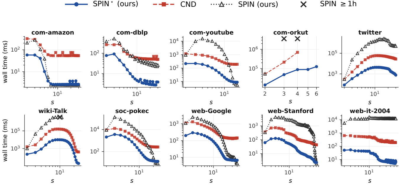
Figure 3: End-to-end time across ten graphs.
